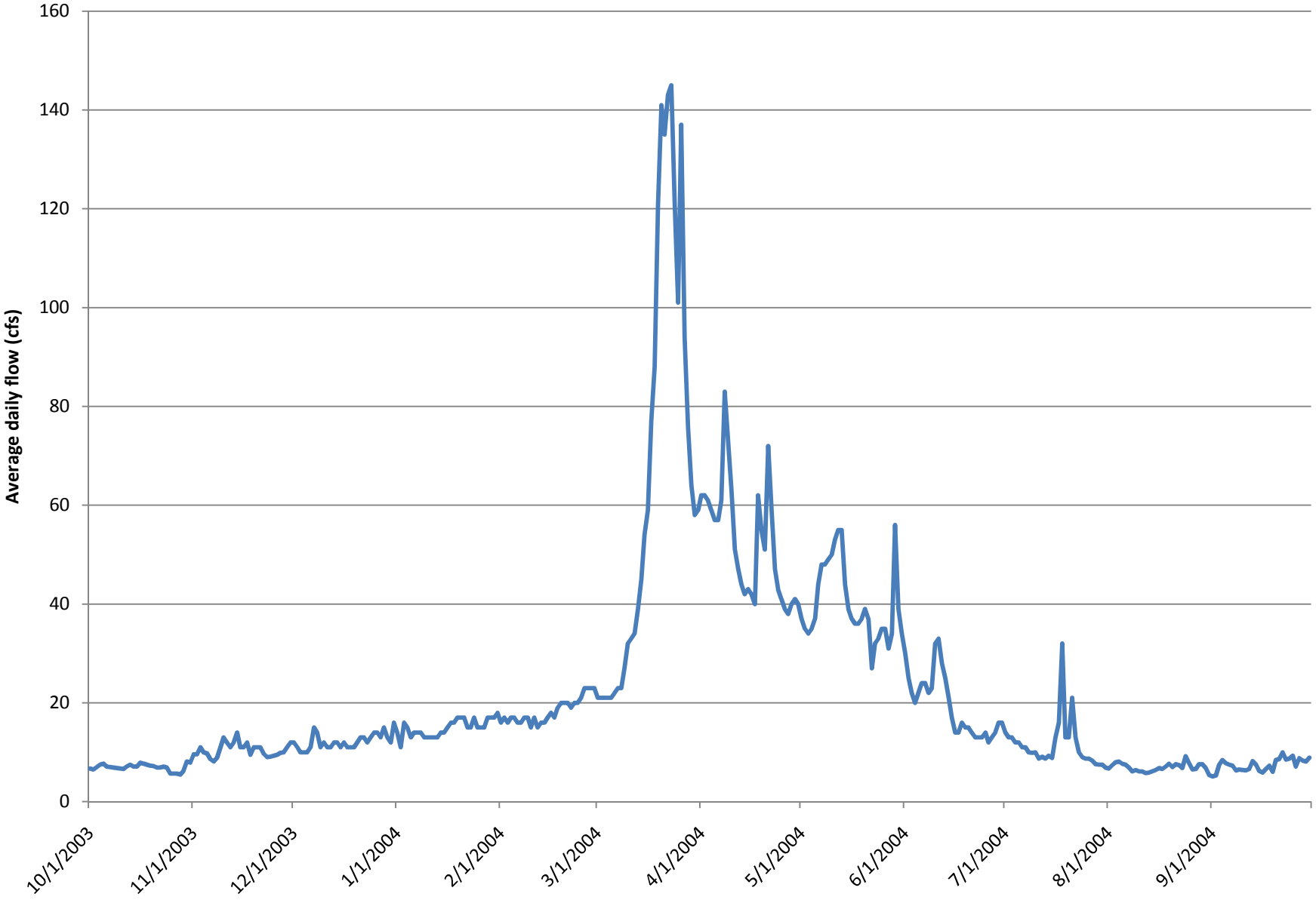
Flow at USGS Gate near Jeremy Ranch (cfs): 2003 - 2004 Water Year
