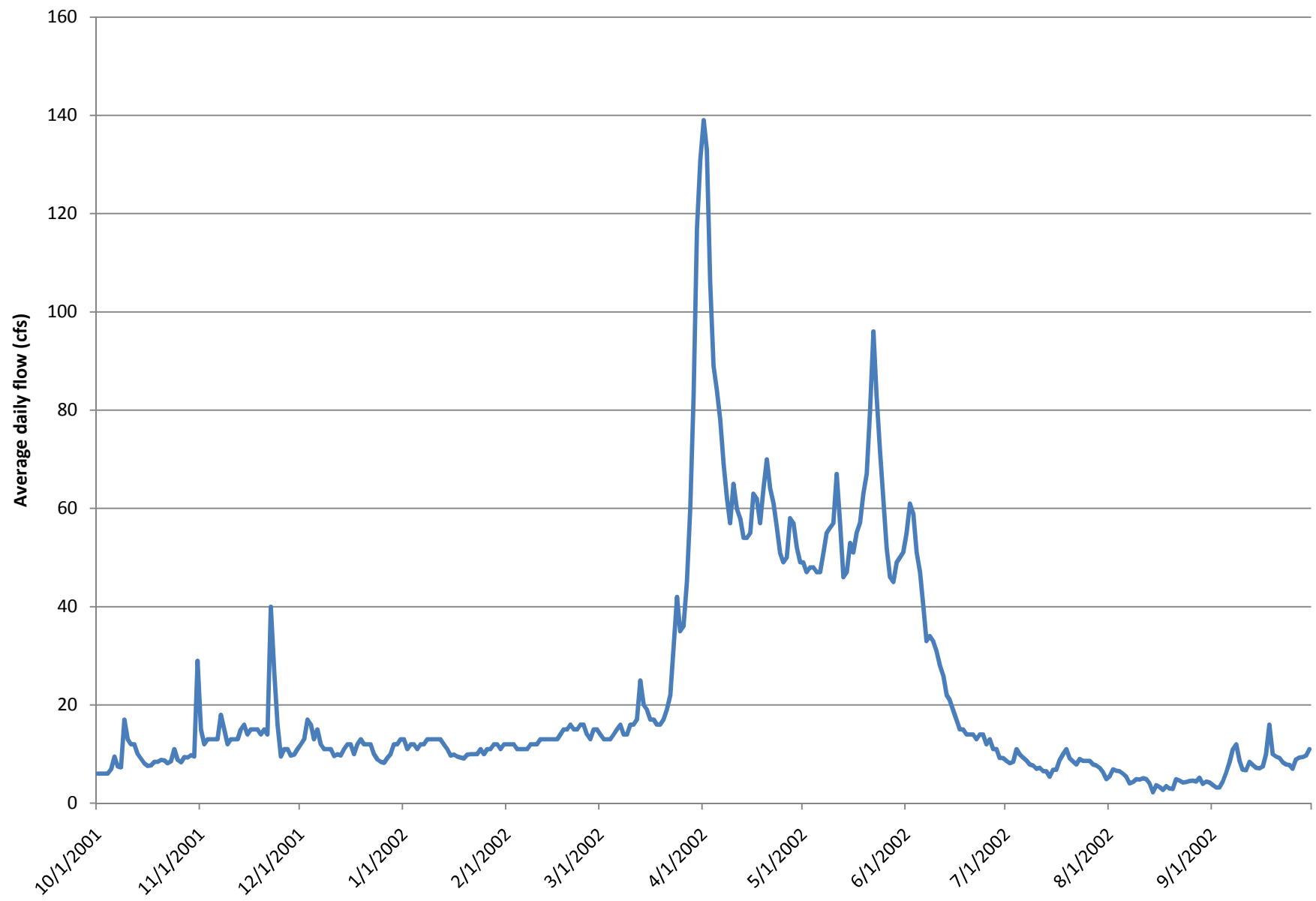
Flow at USGS Gate near Jeremy Ranch (cfs): 2001 - 2002 Water Year
