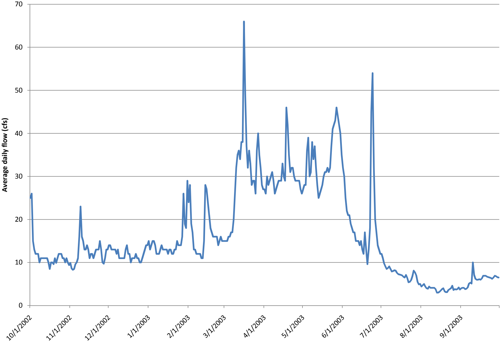
Flow at USGS Gate near Jeremy Ranch (cfs): 2002 - 2003 Water Year
