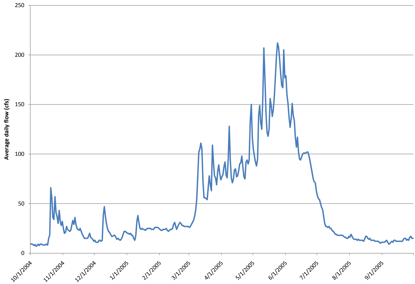
Flow at USGS Gate near Jeremy Ranch (cfs): 2004 - 2005 Water Year
